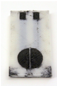
Fig. 5. Resistive Button
